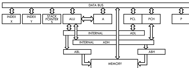
Block Diagram of MCS650X Including Stack Pointer, S FIGURE 8.1
